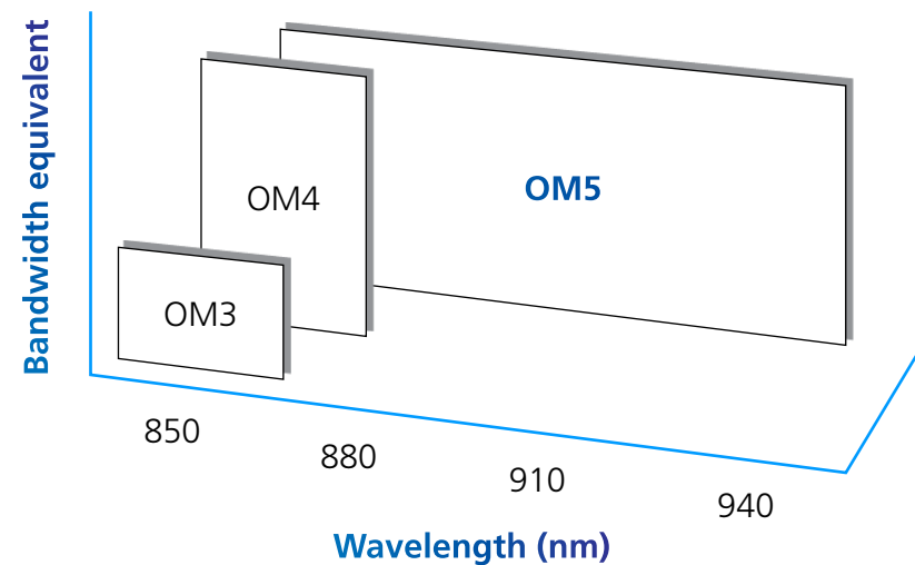
Difference in effective modal bandwidth
