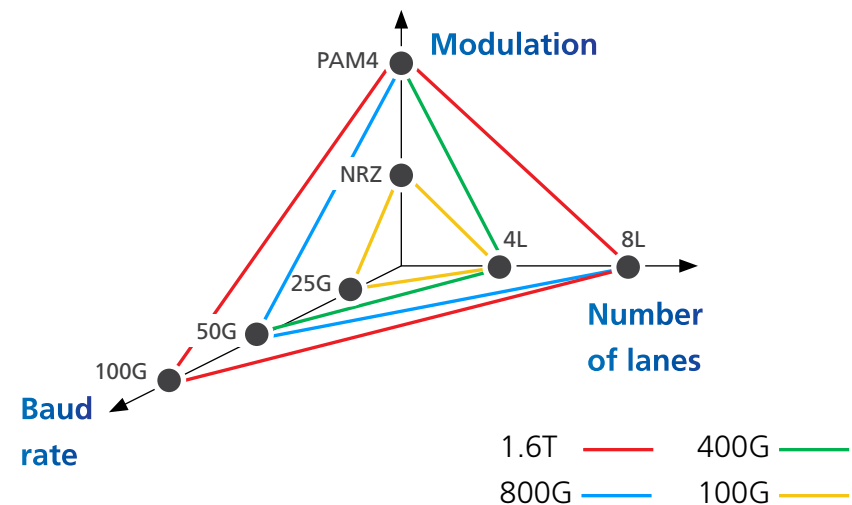
Potential paths to 200G lanes. Source: Marvell
