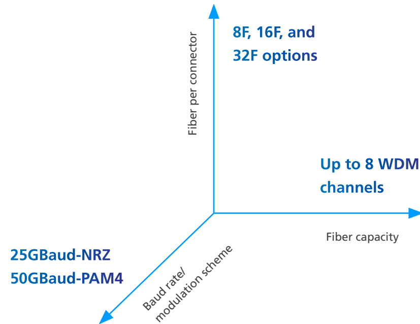
Three paths to higher Ethernet speeds
